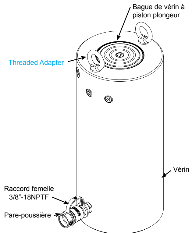
Figure 1 - Composants de vérin type
